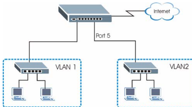
Figure 22 Initial Setup Network Example: VLAN
