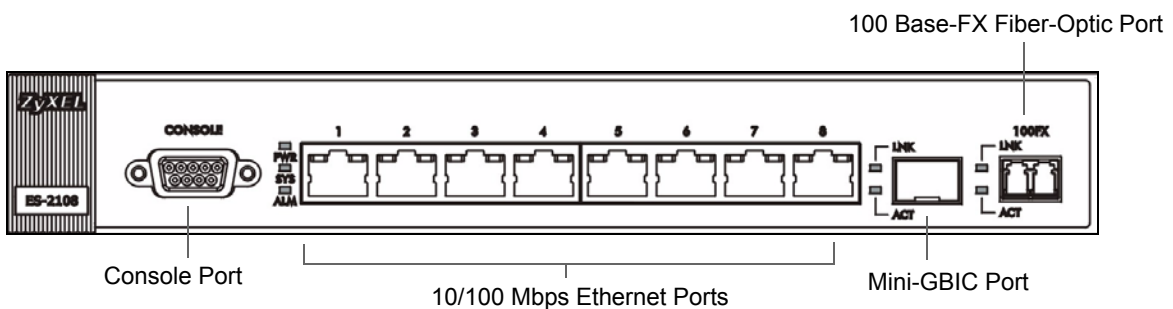
Figure 11 Front Panel: ES-2108-LC
