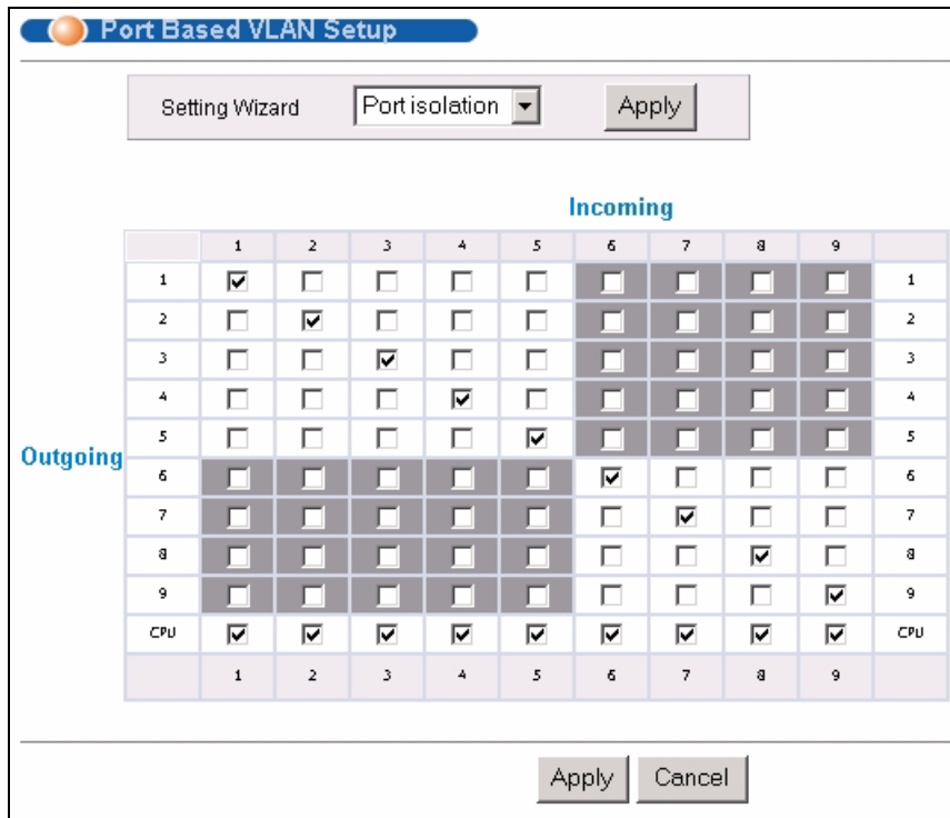
Figure 38 Port Based VLAN Setup (Port Isolation)
