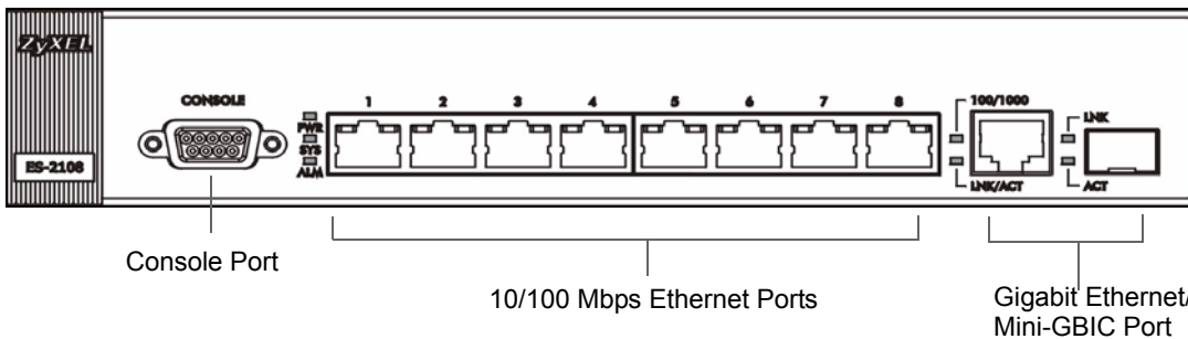
Figure 10 Front Panel: ES-2108-G/ES-2108PWR
