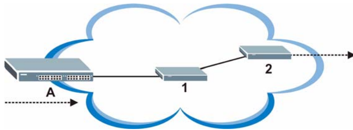
Figure 56 DiffServ Network Example
