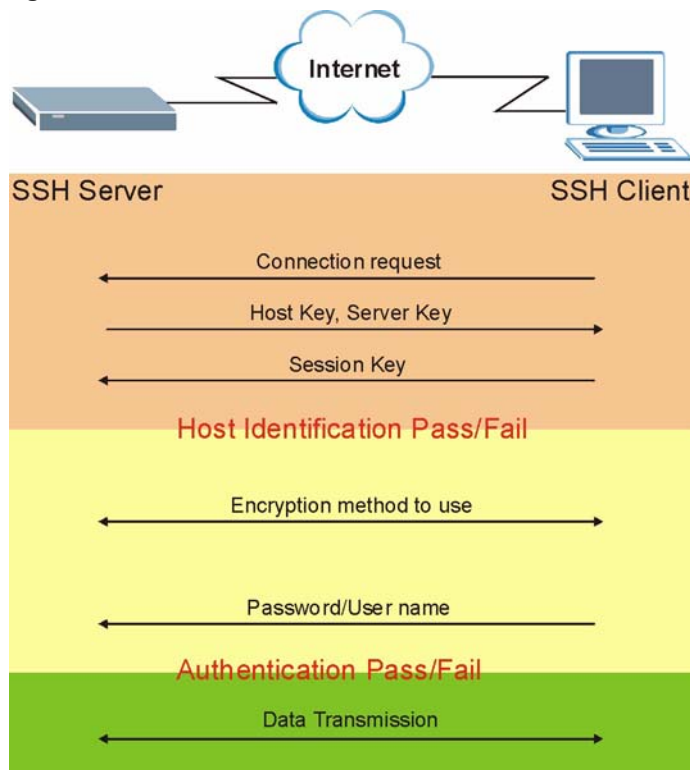
Figure 73 How SSH Works
