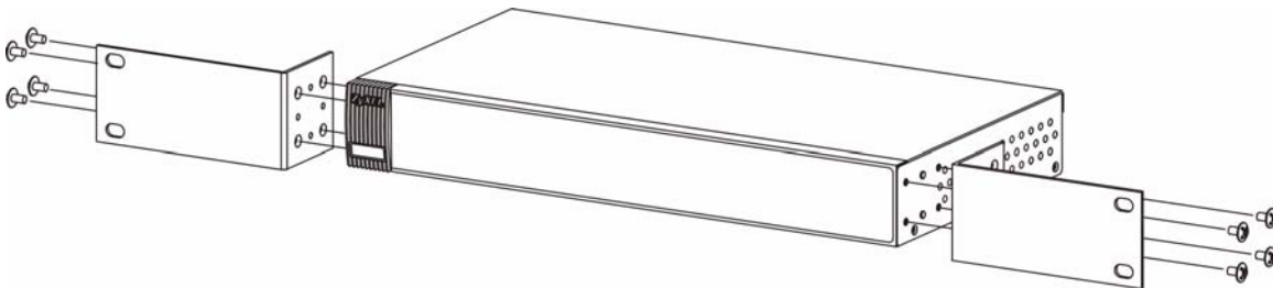
Figure 7 Attaching the Mounting Brackets
