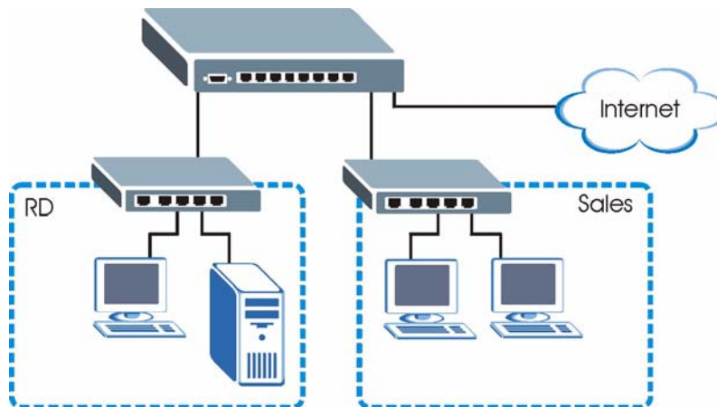
Figure 2 Bridging Application
