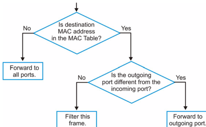
Figure 89 MAC Table Flowchart
