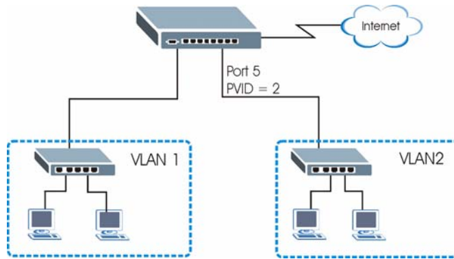
Figure 23 Initial Setup Network Example: Port VID
