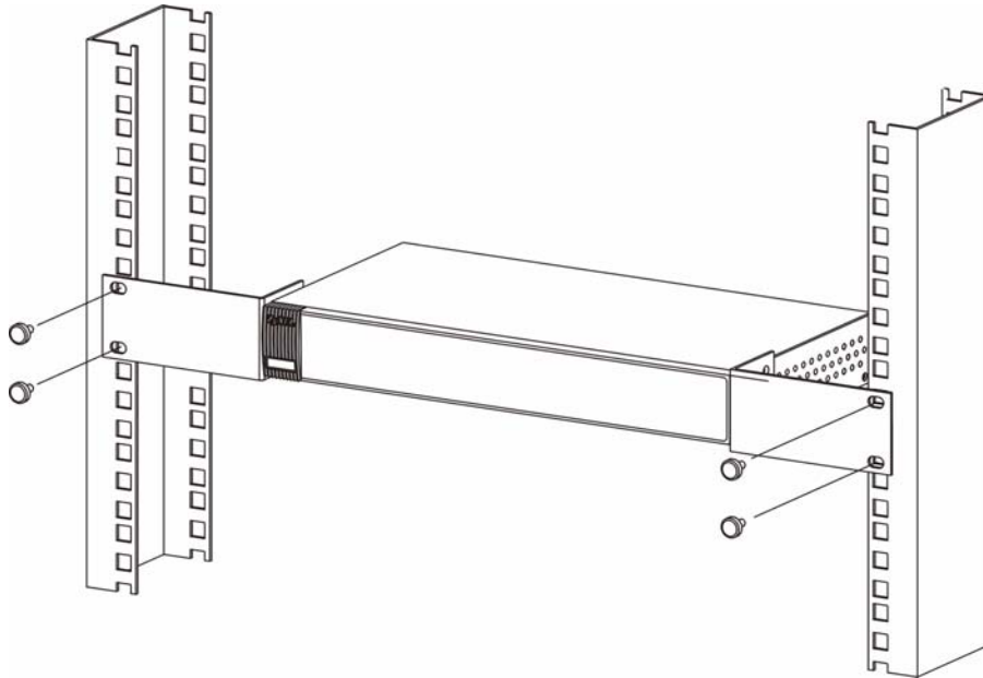
Figure 8 Mounting the Switch on a Rack
