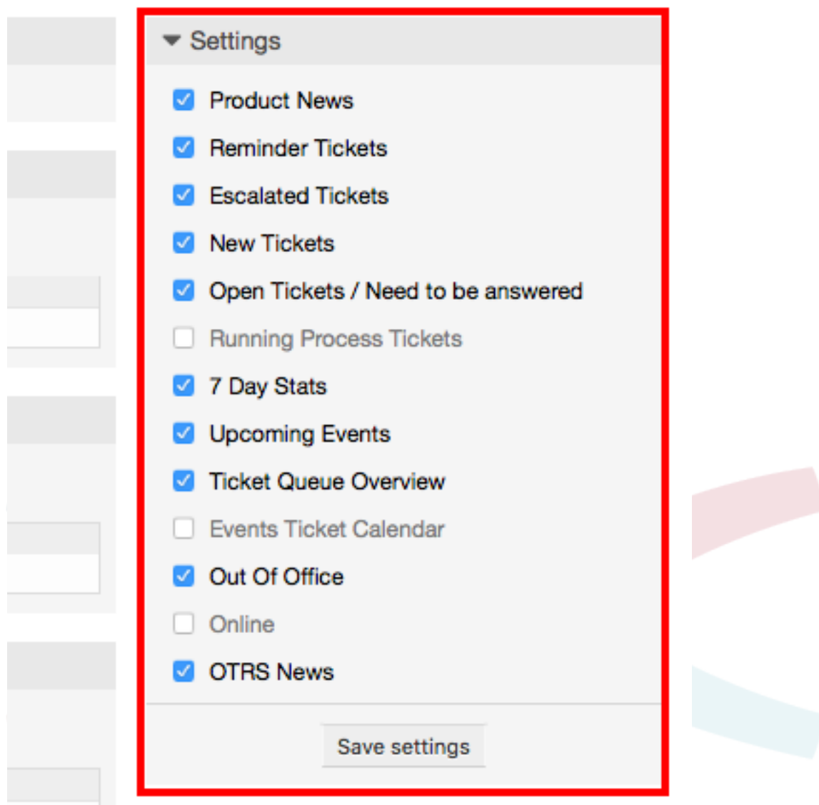
Figure 3.9. Dashboard Settings
