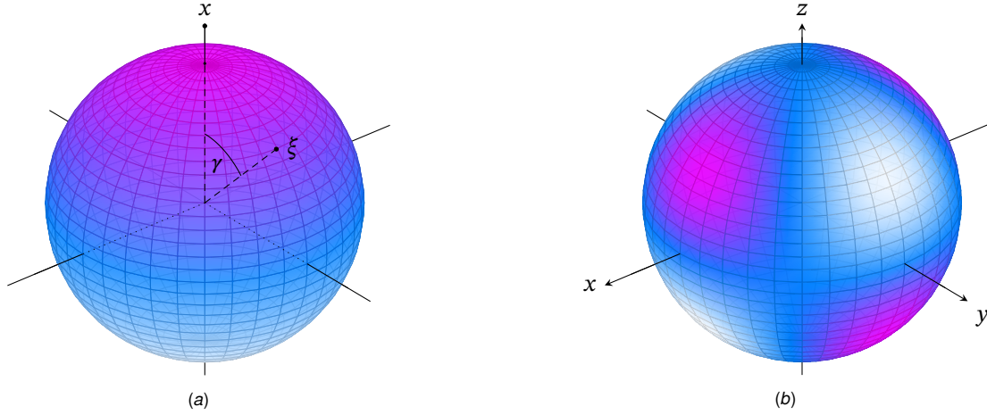
Fig. 1 A figure with two subfigures: (a) Zonal harmonic n = 1, m = 0 , (b) Tesseral harmonic n = 2, m = 3 . See Appendix A.
