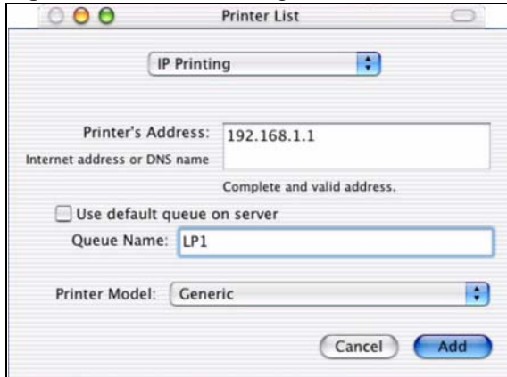
Figure 167 Printer Configuration
