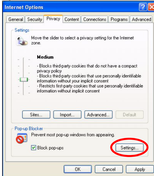
Figure 198 Internet Options
