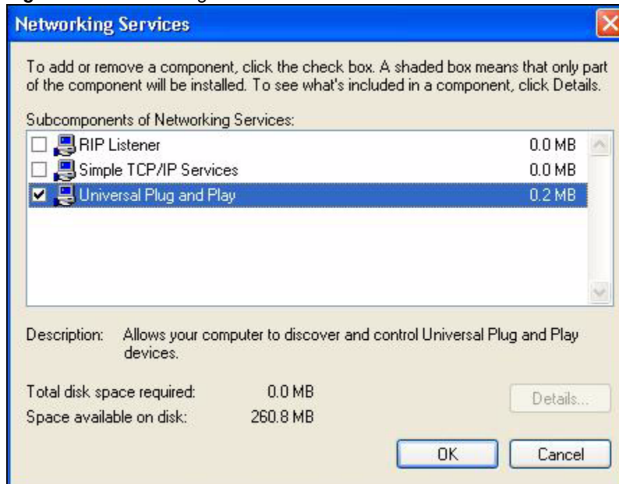
Figure 130 Networking Services
