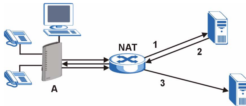
Figure 71 STUN
