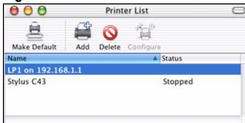
Figure 169 Print Server
