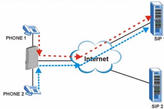
Figure 192 Outgoing Calls: Default
