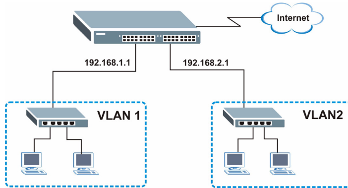
Figure 22 Initial Setup Example: Management IP Address
