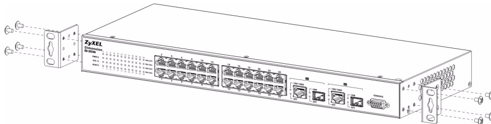
Figure 7 Attaching the Mounting Brackets
