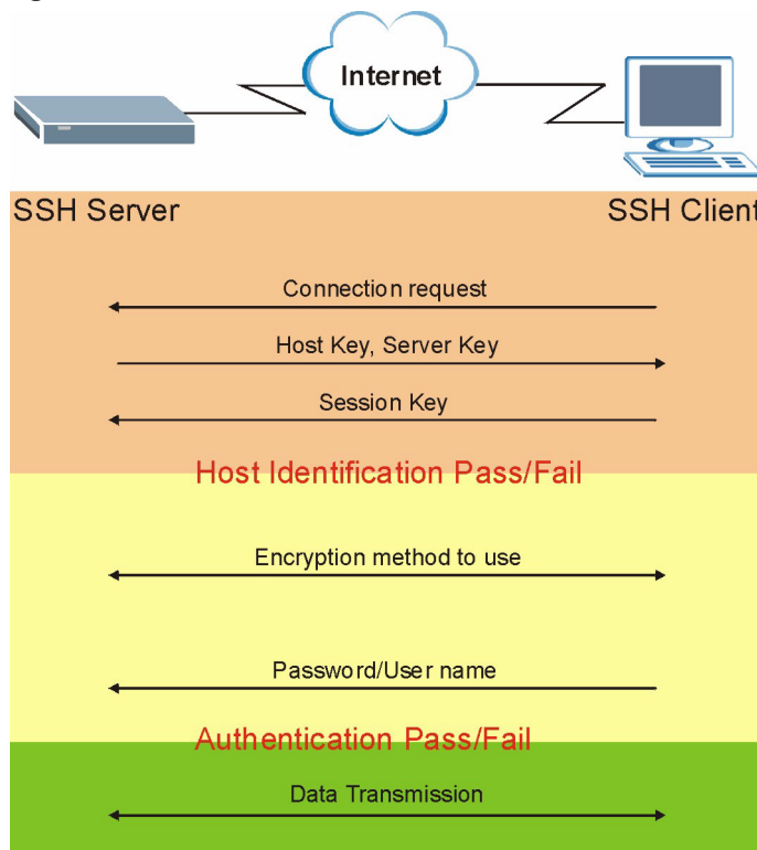
Figure 71 How SSH Works
