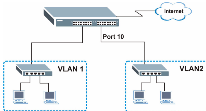
Figure 20 Initial Setup Network Example: VLAN
