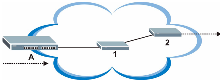
Figure 54 DiffServ Network Example
