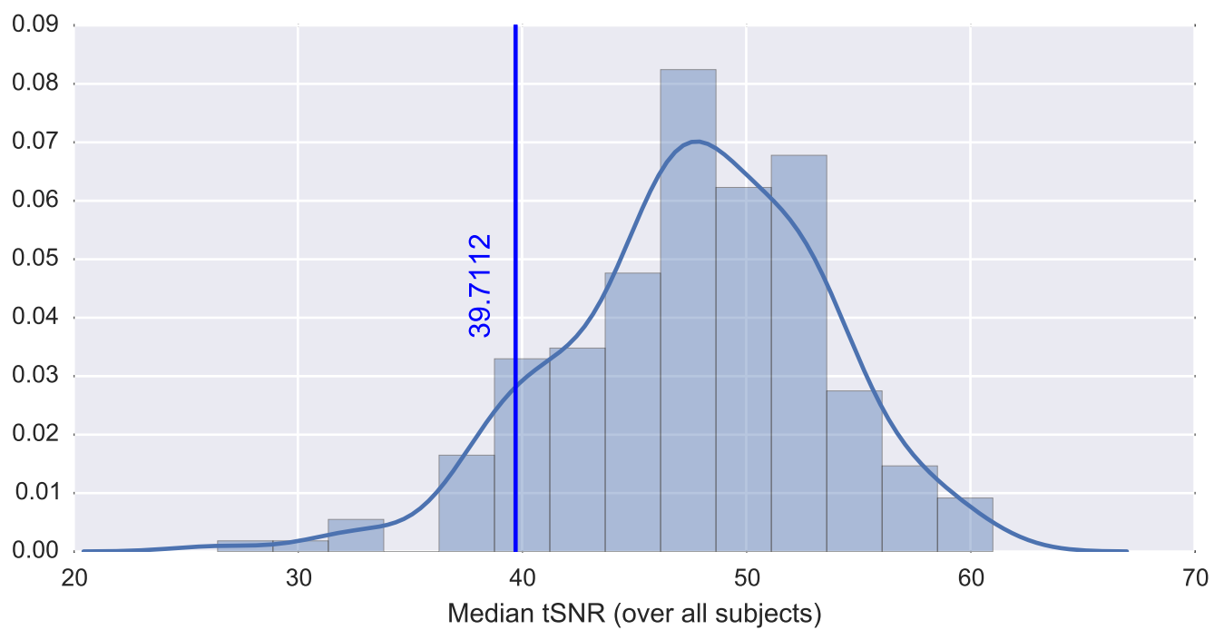
Subject 24944 tSNR inside the mask
