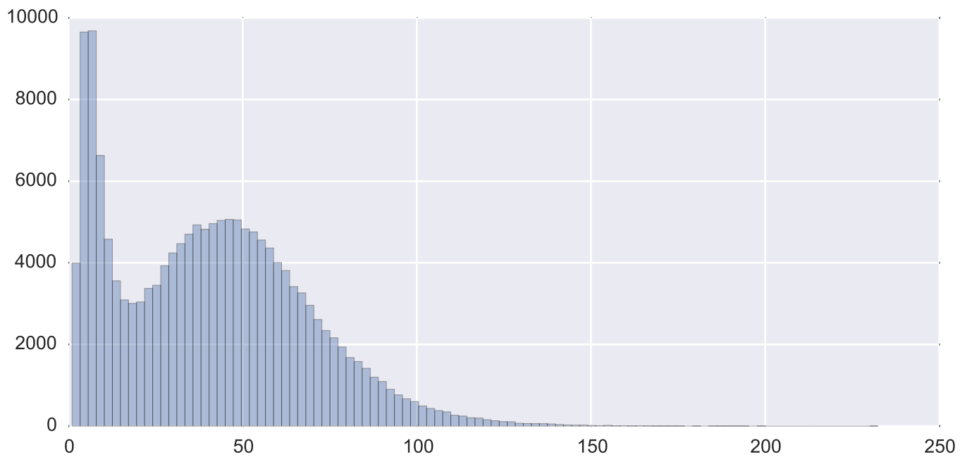
Subject 24944 tSNR inside the mask
