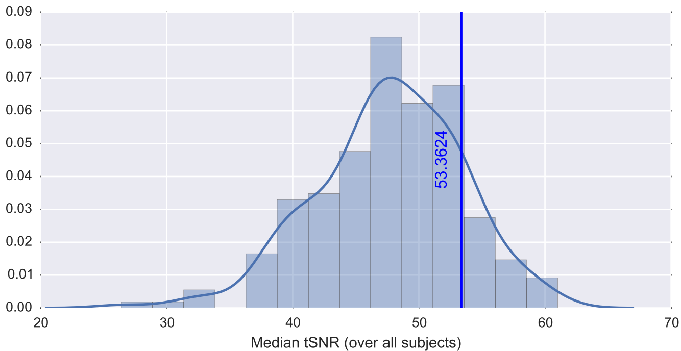
Subject 23197 tSNR inside the mask
