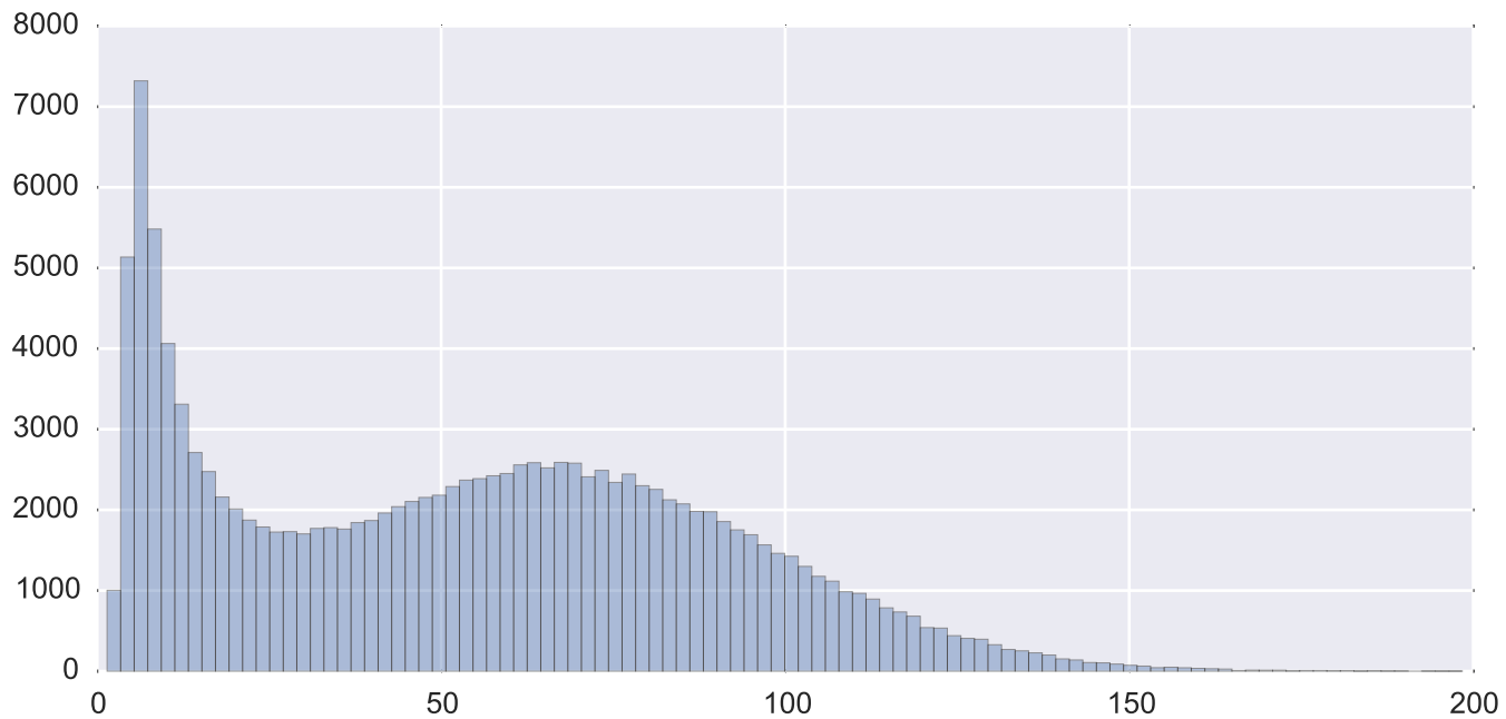
Subject 23197 tSNR inside the mask
